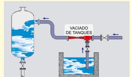
EDUCTORES / EDUCTORS
