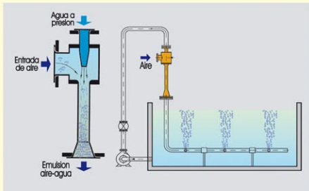
AIREADORES TANQUES / AERATORS FOR TANKS
